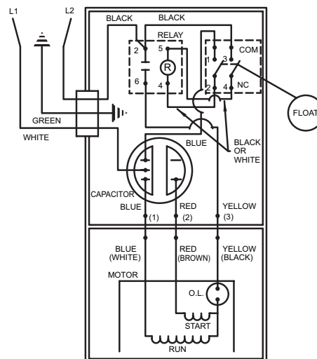
WIRING DIAGRAM FOR MODELS "M161-B", "M161-C", "M161-D", & "M161-E" "D161-B" 9/86 (VS) to Current
