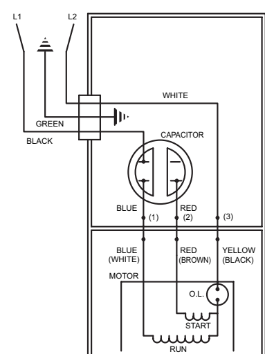
WIRING DIAGRAM FOR MODELS "N161-A", "N161-B", "N161-C", "N161-D", & "N161-E" "E161-A", "E161-B" 2/85 (NR) to Current
